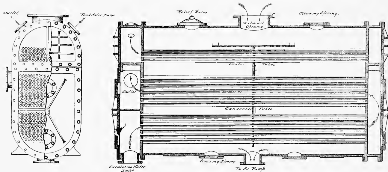
THE VOLZ PATENT COMBINED SURFACE CONDENSER AND FEED-WATER HEATER.
